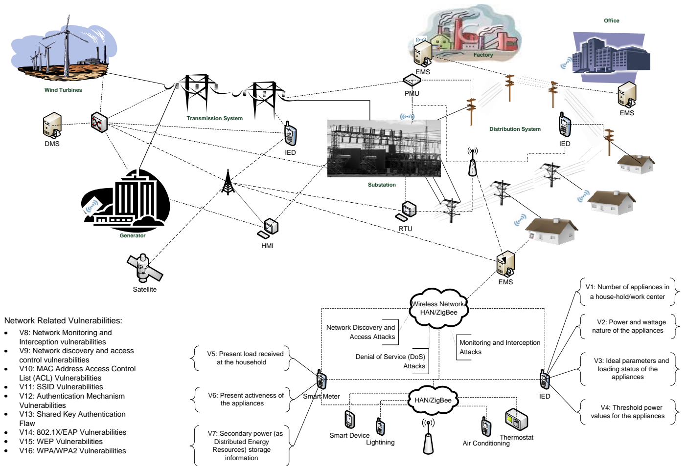
Fig. 2. SG Block Diagram with Communication Network and Devices.
